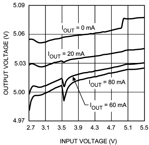
Output Voltage vs. Input Voltage, Version A (5V), 725kHz
