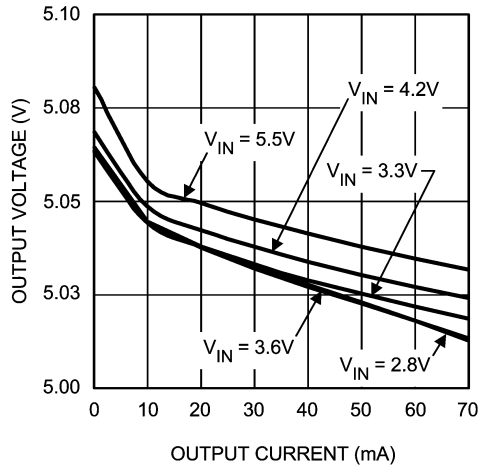
Output Voltage vs. Output Current, Version A (5V), 725kHz
