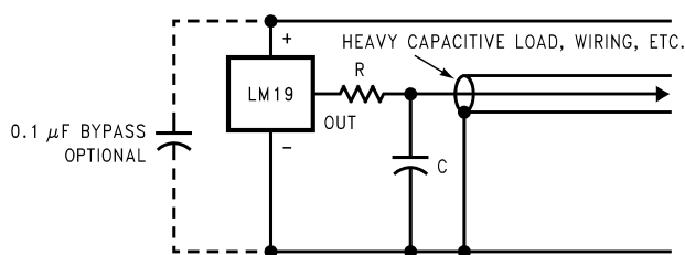
FIGURE 5. LM19 with Filter for Noisy Environment and Capacitive Loading greater than 300 pF. Either placement of resistor as shown above is just as effective.
