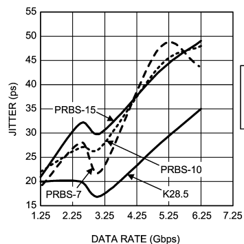
Total Jitter vs Data Rate For 10in of FR4 Board (Input Level = 1V_{P-P} )
