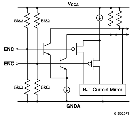
FIGURE 3. CLC5957 ENCODE Clock Inputs
