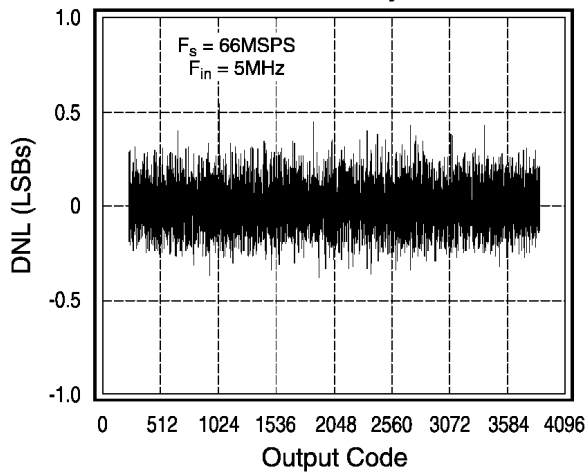
Differential Non-Linearity
