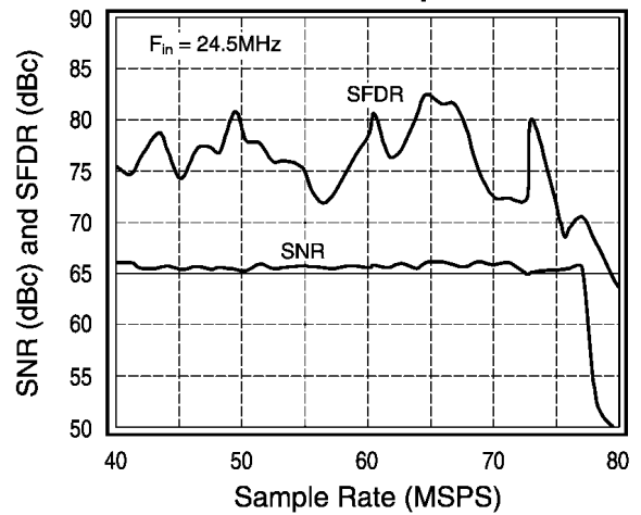
SNR and SFDR vs. Sample Rate
