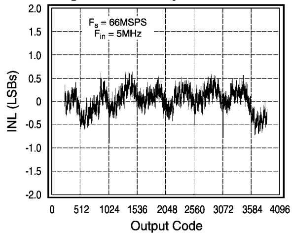
Integral Non-Linearity
