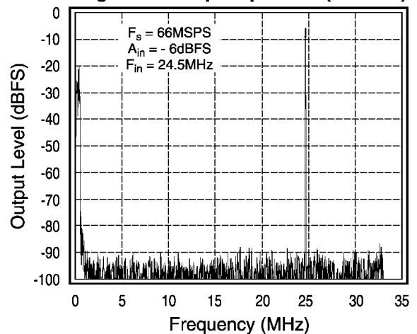
Single Tone Output Spectrum (w/Dither)
