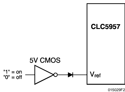
FIGURE 2. Power Shutdown Scheme
