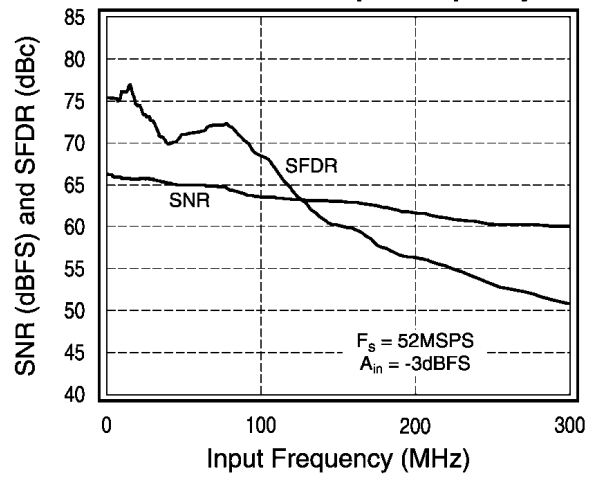
SNR and SFDR vs. Input Frequency
