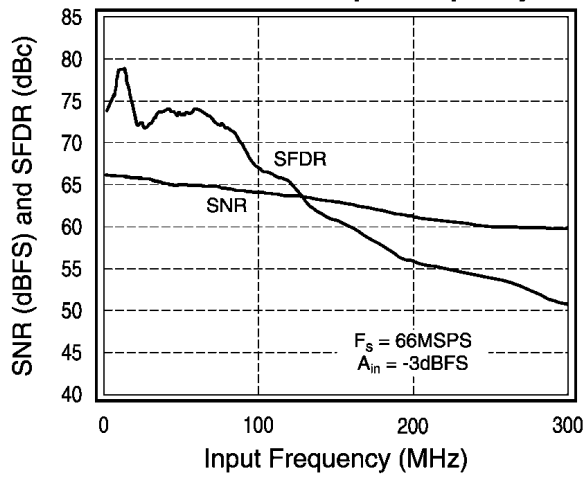
SNR and SFDR vs. Input Frequency
