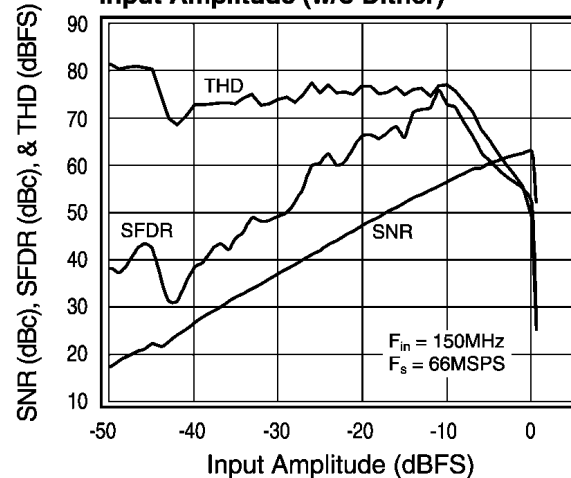
SNR and SFDR vs. Input Amplitude (w/o Dither)
