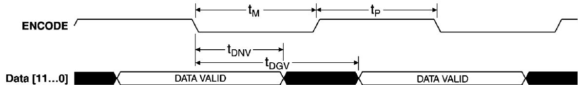
CLC5957 ENCODE to Data Timing Diagram
