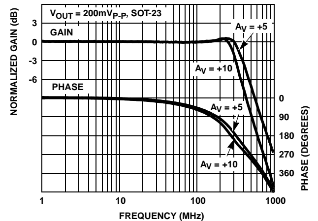
FIGURE 17. FREQUENCY RESPONSE
