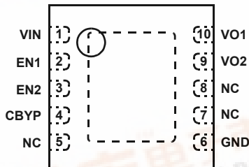
ISL9014 10 LD 3X3 DFN TOP VIEW
