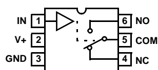
ISL84544 (SOT-23) TOP VIEW
