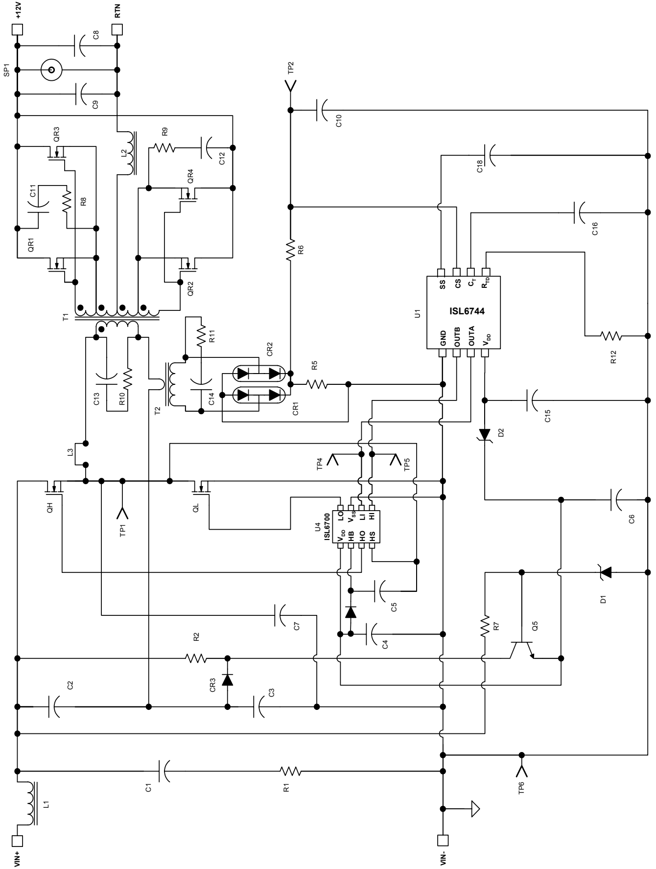
Typical Application using ISL6744 - 48V Input DC Transformer, 12V @ 8A Output
