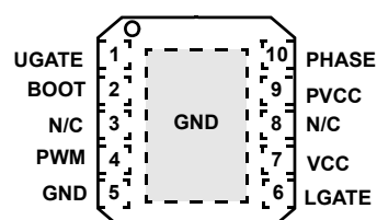
ISL6612BCR, ISL6613BCR (10L 3x3 DFN) TOP VIEW
