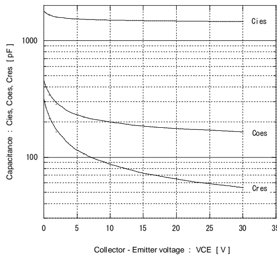
[ Brake ] Capacitance vs. Collector-Emitter voltage (typ.) V_{GE} = 0V, f = 1\text{MHz}, T_j = 25^\circ\text{C}
