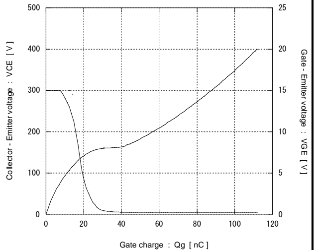
[ Brake ] Dynamic Gate charge (typ.) V_{cc} = 300V, I_c = 15A, T_j = 25^\circ\text{C}
