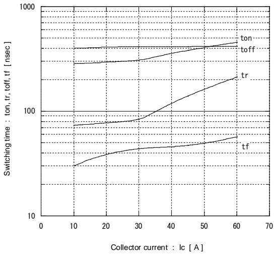
[ Inverter ] Switching time vs. Collector current (typ.) Vcc=300V, VGE=+15V, Rg=68Ω, Tj= 25°C
