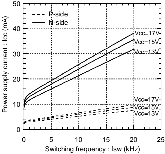
Power supply current vs. Switching frequency T_c=125^\circ\text{C} (typ.)
