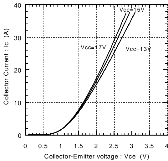
Collector current vs. Collector-Emitter voltage (typ.) T j =25°C
