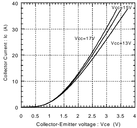
Collector current vs. Collector-Emitter voltage (typ.) T j =125°C
