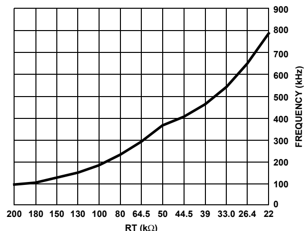
FIGURE 3. FREQUENCY vs RT
