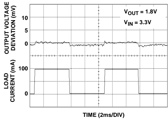
FIGURE 6. LOAD REGULATION RESPONSE ( V_{OUT1} )
