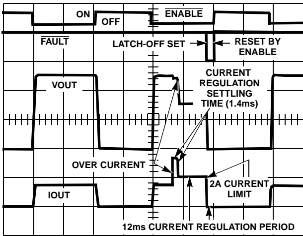
FIGURE 2. OPERATIONAL WAVEFORMS
