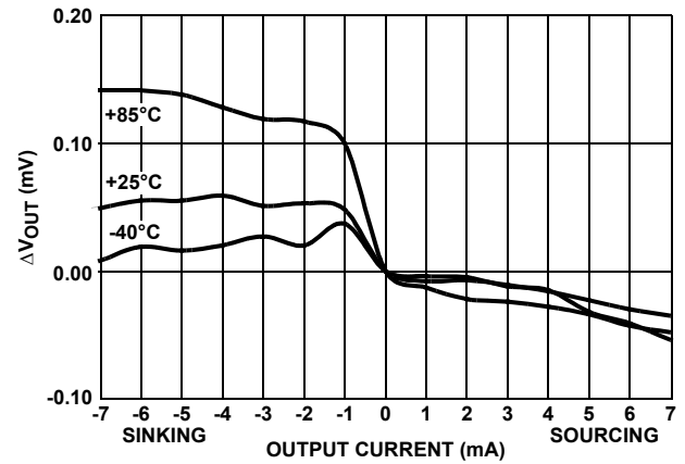
FIGURE 79. LOAD REGULATION
