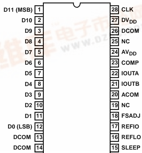
ISL5861 TOP VIEW
