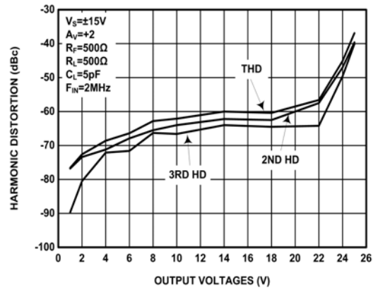
FIGURE 18. HARMONIC DISTORTION vs OUTPUT VOLTAGE ( A_V = +2 )
