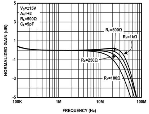
FIGURE 12. GAIN vs FREQUENCY FOR VARIOUS R_{FEEDBACK} ( A_V = +2 )
