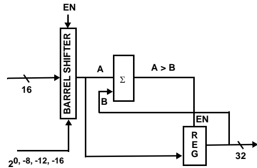
FIGURE 2. PEAK DETECTOR
