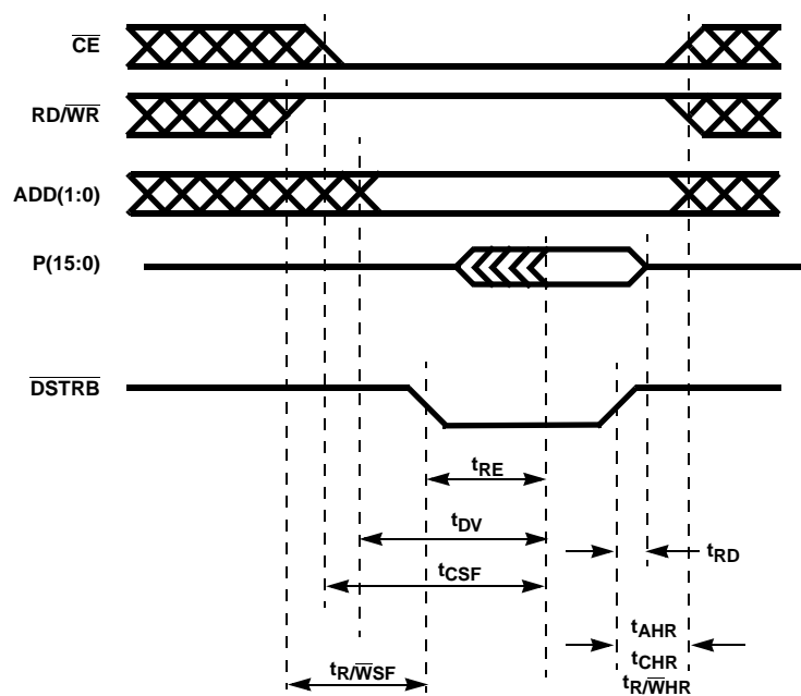
FIGURE 10. MICROPROCESSOR READ TIMING ( \mu P MODE = 1)
