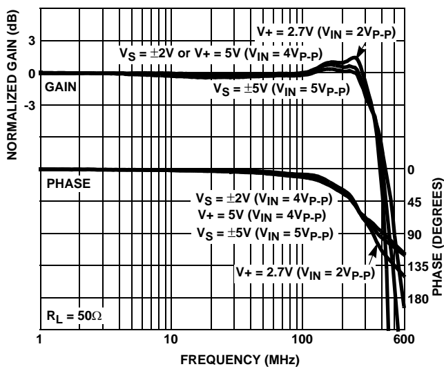
FIGURE 19. FREQUENCY RESPONSE
