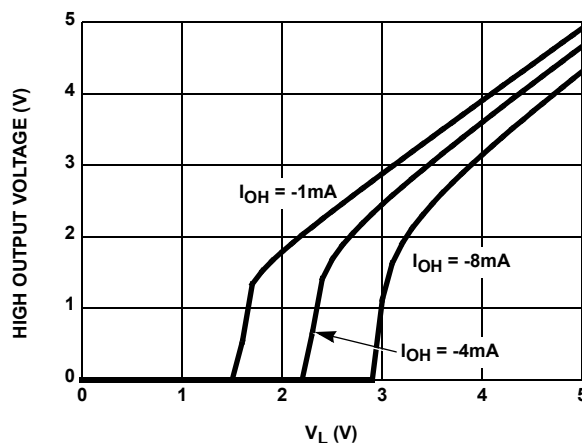
FIGURE 14. RECEIVER HIGH OUTPUT VOLTAGE vs LOGIC SUPPLY VOLTAGE ( V_L )
