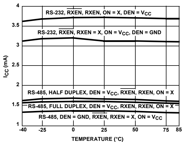
FIGURE 18. SUPPLY CURRENT vs TEMPERATURE
