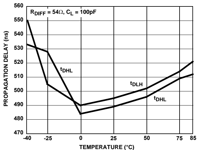
FIGURE 23. RS-485, DRIVER PROPAGATION DELAY vs TEMPERATURE (MEDIUM DATA RATE, QFN ONLY)
