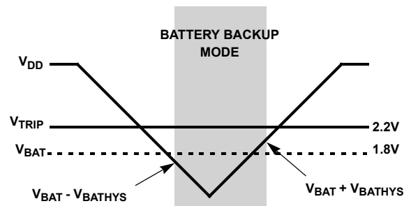
FIGURE 13. BATTERY SWITCHOVER WHEN V_{\text{BAT}} < V_{\text{TRIP}}
