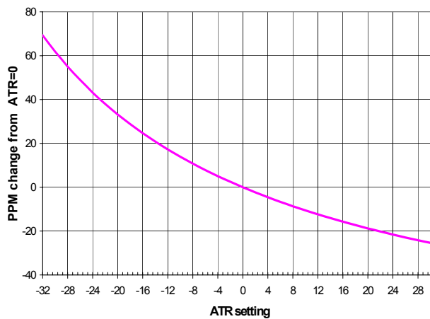
FIGURE 10. \Delta F_{OUT} vs ATR SETTING
