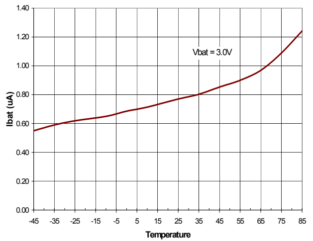
FIGURE 8. I_{BAT} vs TEMPERATURE
