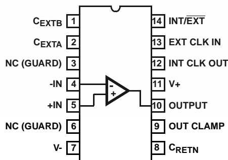
ICL7650S (PDIP) TOP VIEW
