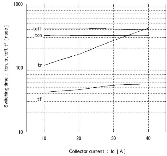
[ Inverter ] Switching time vs. Collector current (typ.) Vcc=300V, VGE=+15V, Rg=150Ω, Tj= 125°C
