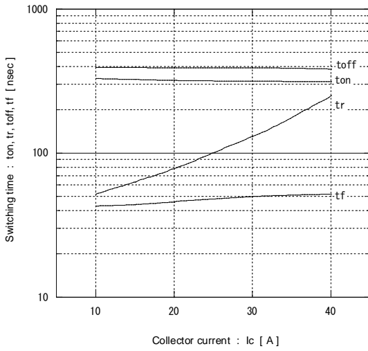
[ Inverter ] Switching time vs. Collector current (typ.) Vcc=300V, VGE=+15V, Rg=150Ω, Tj= 25°C
