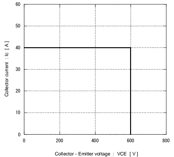
[ Inverter ] Reverse bias safe operating area (max) +VGE=15V, -VGE<=15V, Rg=>150Ω, Tj<=125°C
