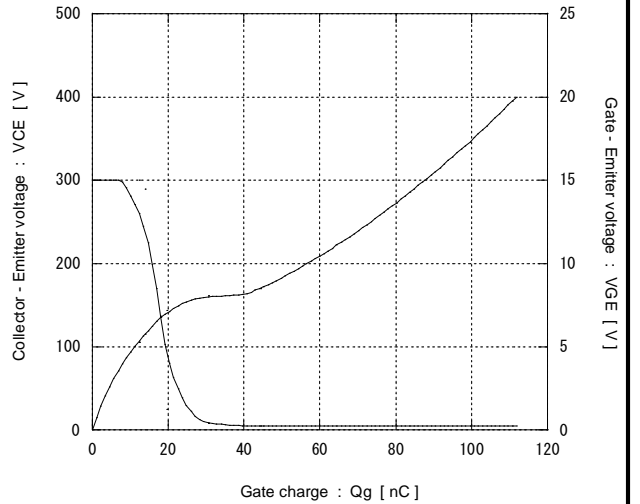
[ Inverter ] Dynamic Gate charge (typ.) V CC =300V, I c =15A, T j = 25°C
