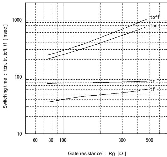
[ Inverter ] Switching time vs. Gate resistance (typ.) Vcc=300V, Ic=20A, VGE=+15V, Tj= 25°C
