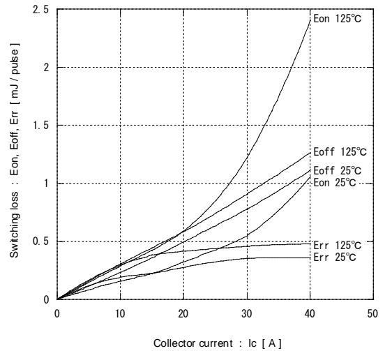
[ Inverter ] Switching loss vs. Collector current (typ.) Vcc=300V, VGE=+15V, Rg=150Ω
