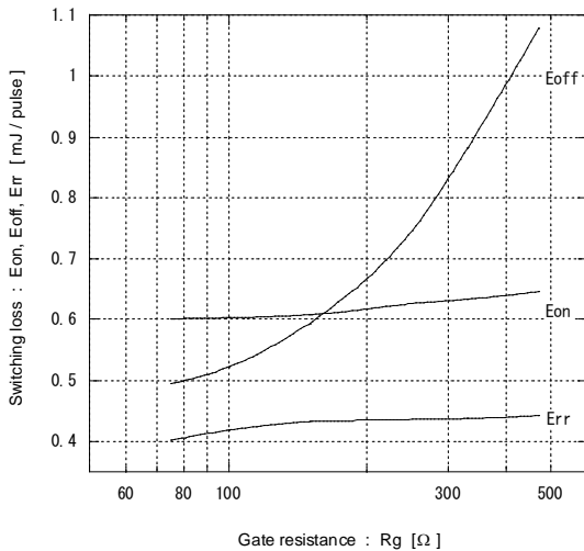
[ Inverter ] Switching loss vs. Gate resistance (typ.) Vcc=300V, Ic=20A, VGE=+15V, Tj= 125°C
