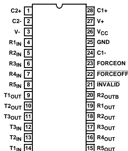
ICL3244 (SSOP) TOP VIEW
