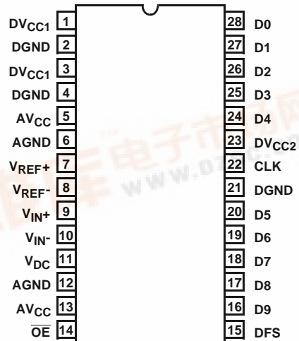
HI5766 (SOIC, SSOP) TOP VIEW
