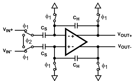
FIGURE 24. ANALOG INPUT SAMPLE-AND-HOLD
