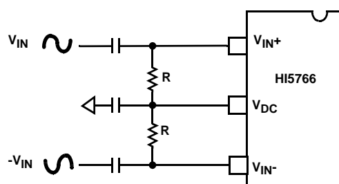
FIGURE 25. AC COUPLED DIFFERENTIAL INPUT
