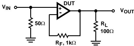
FIGURE 2. SMALL SIGNAL PULSE RESPONSE CIRCUIT
