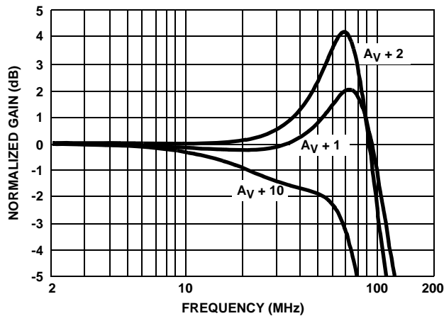
FIGURE 39. NON-INVERTING FREQUENCY RESPONSE
