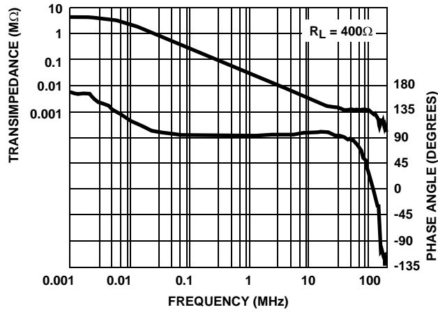
FIGURE 57. TRANSIMPEDENCE vs FREQUENCY
