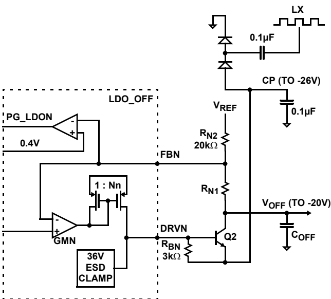
FIGURE 29. V_{OFF} FUNCTIONAL BLOCK DIAGRAM
