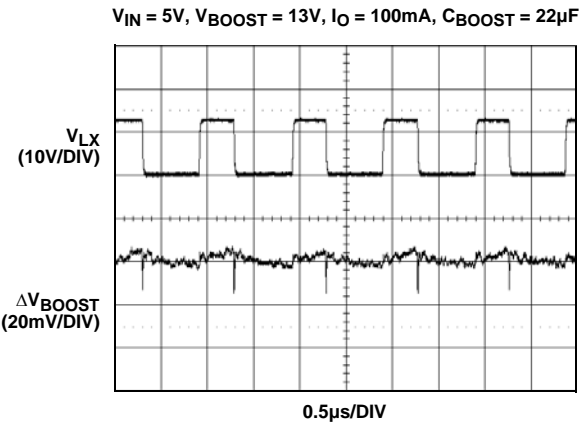
FIGURE 15. BOOST STAGE
