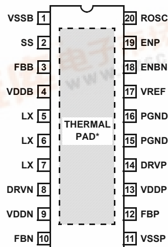
EL7581 (20-PIN HTSSOP) TOP VIEW
