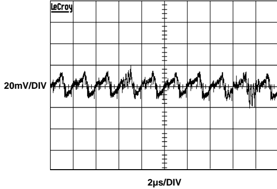
FIGURE 19. V_{OFF} RIPPLE
