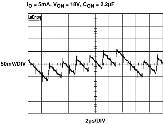
FIGURE 16. V_{ON} RIPPLE
