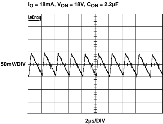
FIGURE 17. V_{ON} RIPPLE
