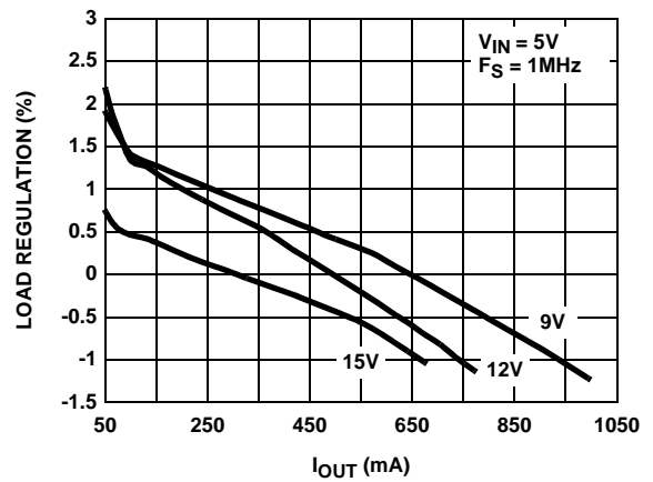
FIGURE 6. LOAD REGULATION
