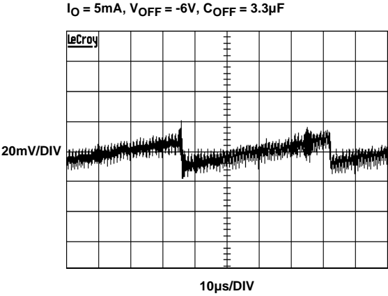
FIGURE 18. V_{OFF} RIPPLE
