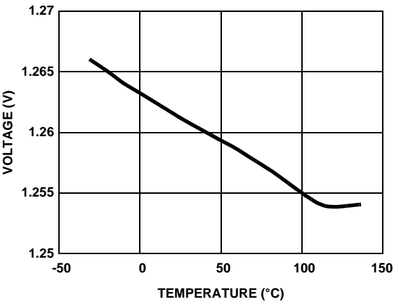
FIGURE 14. V_{REF} vs TEMPERATURE
