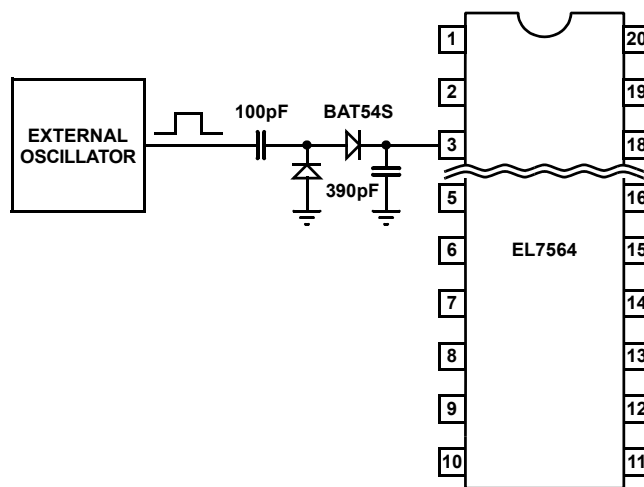
FIGURE 23. OSCILLATOR SYNCHRONIZATION
