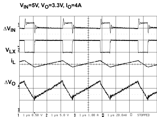
FIGURE 14. SWITCHING WAVEFORMS
