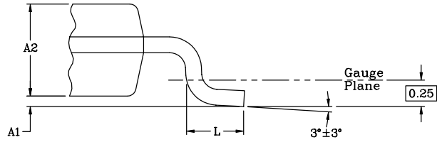
DETAIL X
