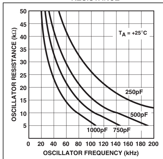
FIGURE 3-8: OSCILLATOR FREQUENCY VS. OSCILLATOR RESISTANCE
