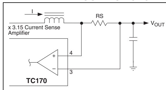
FIGURE 3-3: ABOVE GROUND RESISTIVE SENSING
