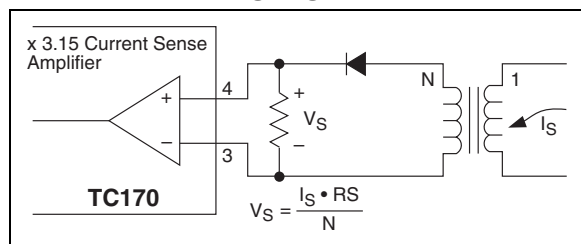
FIGURE 3-4: TRANSFORMER ISOLATED CURRENT SENSE
