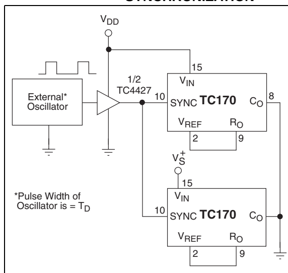
FIGURE 3-6: EXTERNAL CLOCK SYNCHRONIZATION
