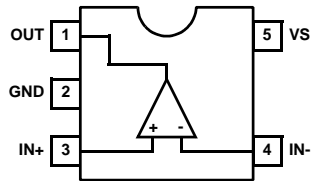
EL5144 (5-PIN SOT-23) TOP VIEW
