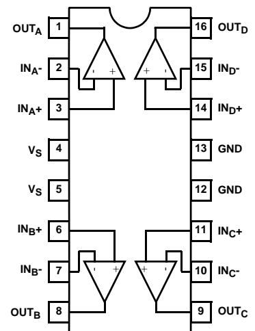
EL5444 (16-PIN QSOP) TOP VIEW
