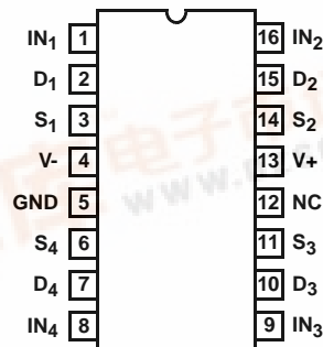
DG441, DG442 (PDIP, SOIC) TOP VIEW
