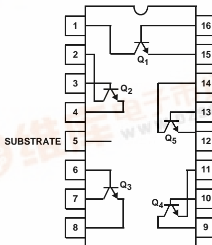
CA3083 (PDIP, SOIC) TOP VIEW
