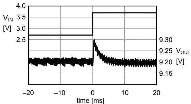
4-5. f_{OSC} = 286\text{ kHz} , V_{IN} = 2.7\text{ V} \rightarrow 3.7\text{ V}
