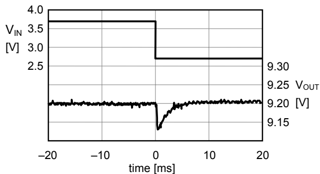
4-4. f_{OSC} = 700\text{ kHz} , V_{IN} = 3.7\text{ V} \rightarrow 2.7\text{ V}
