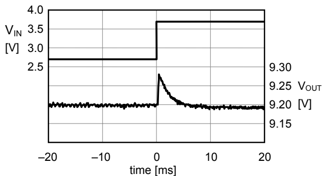
4-3. f_{OSC} = 700\text{ kHz} , V_{IN} = 2.7\text{ V} \rightarrow 3.7\text{ V}
