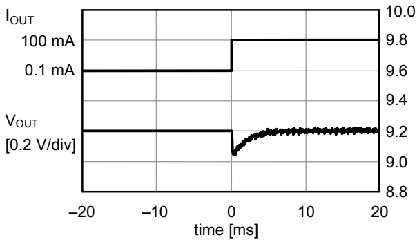
3-5. f_{OSC} = 286\text{ kHz} , I_{OUT} = 0.1\text{ mA} \rightarrow 100\text{ mA}
