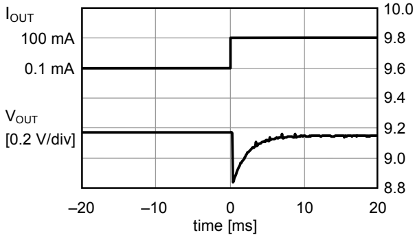
3-3. f_{OSC} = 700\text{ kHz} , I_{OUT} = 0.1\text{ mA} \rightarrow 100\text{ mA}
