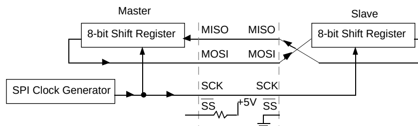
Figure 8-3. Serial Peripheral Interface Master-Slave Interconnection
