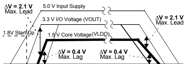
Figure 19. Inverted Power Up/Down Sequence in +5.0 V Supply System
