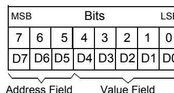
Figure 23. Command Byte
