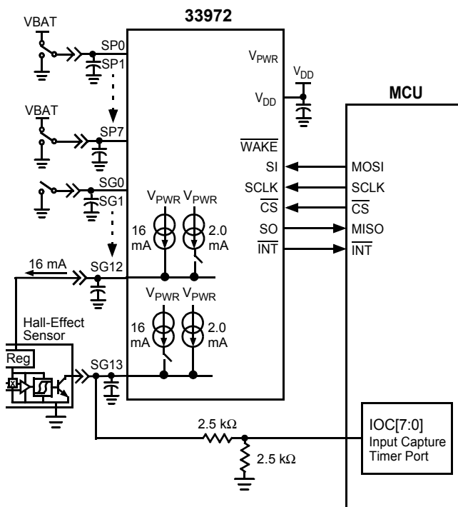
Figure 12. Sensor Power Supply
