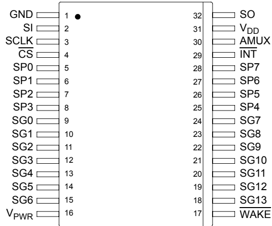
Figure 3. 33972 Terminal Connections
