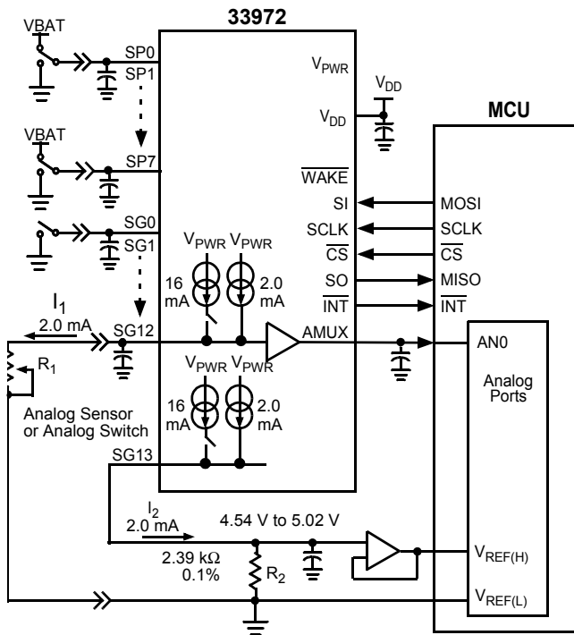
Figure 13. Analog Ratiometric Conversion
