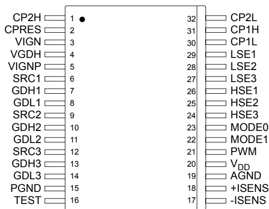
Figure 3. 33395 Terminal Connections
