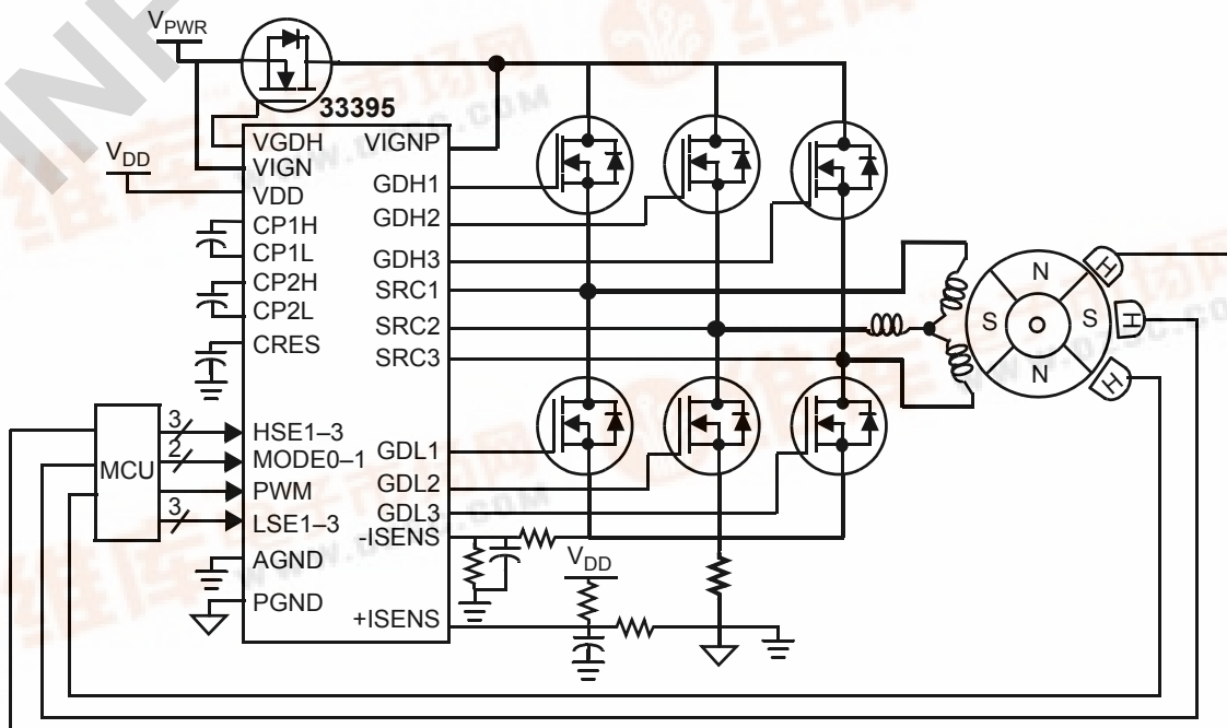
Figure 1. 33395 Simplified Application Diagram
