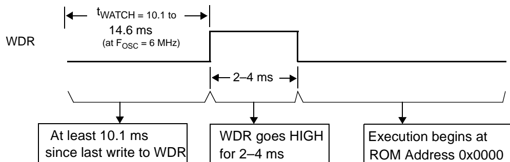
Figure 10-1. Watchdog Reset (WDR, Address 0x26)
