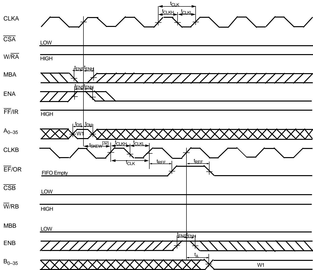
EF Flag Timing and First Data Read Fall Through when FIFO is Empty (CY Standard Mode) [30]
