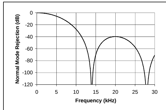
FIGURE 4-2: SINC Filter Magnitude Response ( \text{MCLK} = 3.58\text{ MHz} ).
