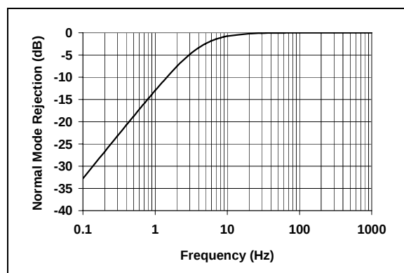
FIGURE 4-4: HPF Magnitude Response ( MCLK = 3.58 MHz).
