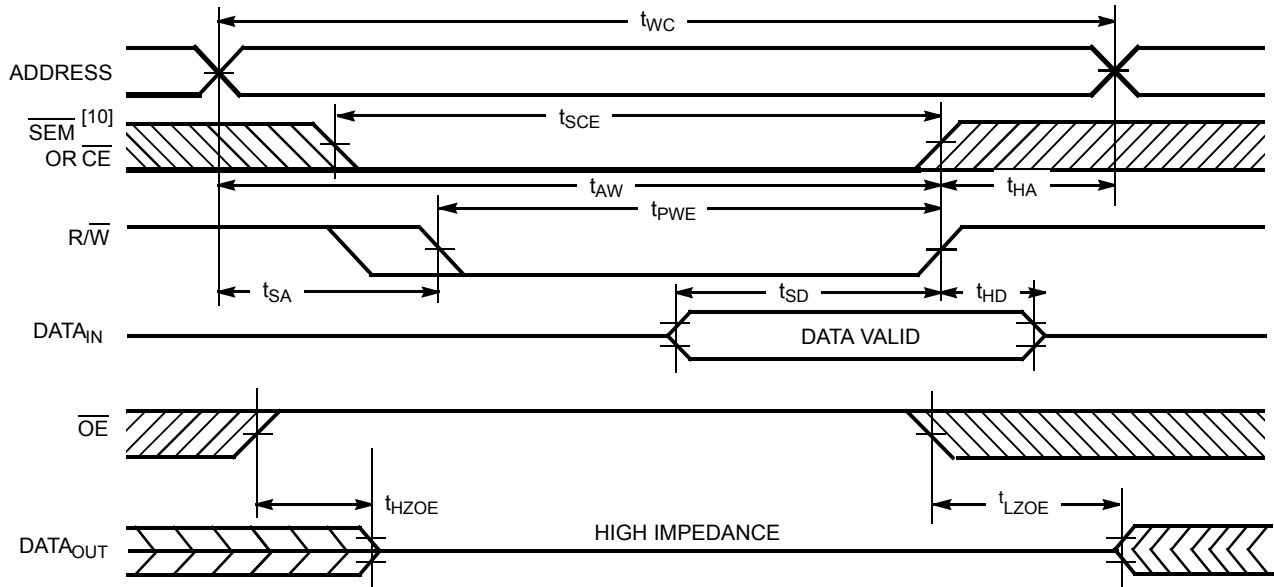
Write Cycle No. 2: \overline{R/\overline{W}} Three-States Data I/Os (Either Port) [16, 18]
