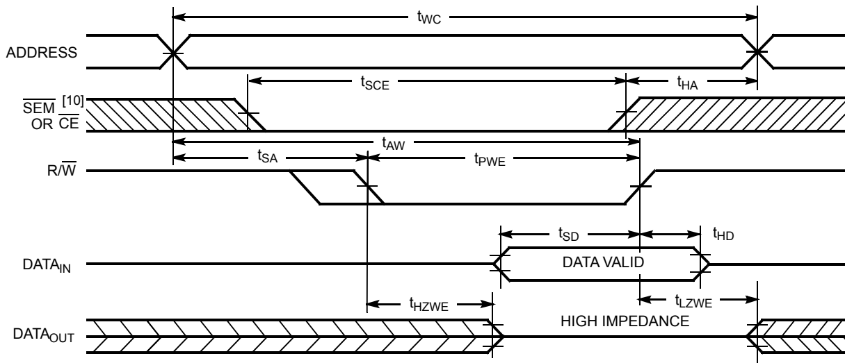
Write Cycle No. 2: \overline{R/\overline{W}} Three-States Data I/Os (Either Port) [16, 18]
