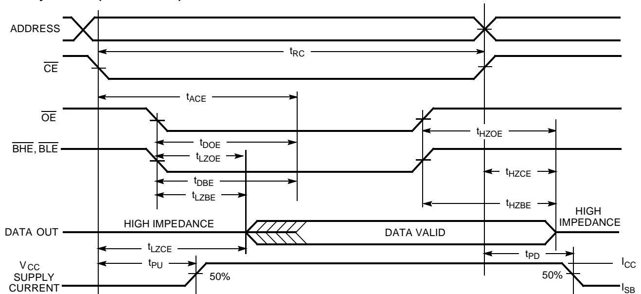
Read Cycle No. 2 ( \overline{OE} Controlled) [9, 10]
