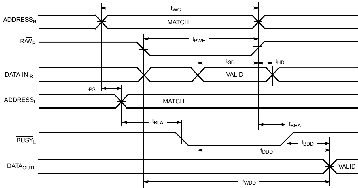
Timing Diagram of Write with \overline{\text{BUSY}} ( M/\overline{S} = \text{HIGH} ) [41]
