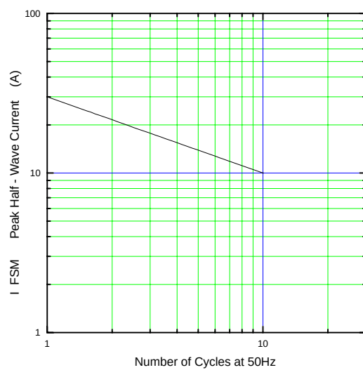
Surge Capability
