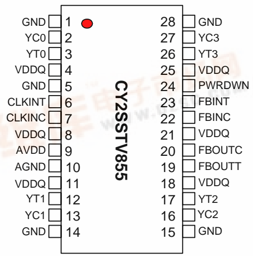
28-pin TSSOP
