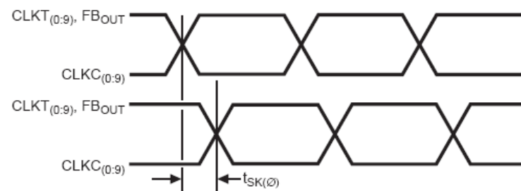
Figure 7. Output Skew
