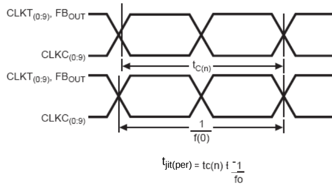
Figure 3. Period Jitter
