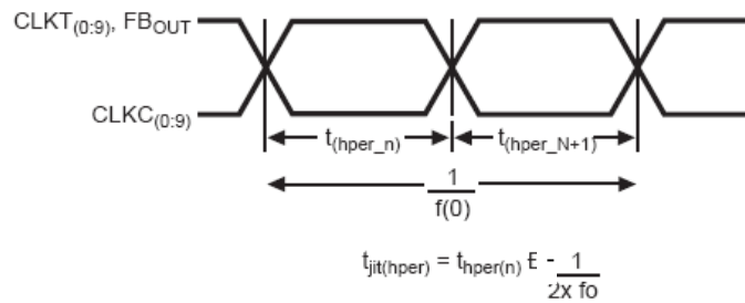
Figure 4. Half Period Jitter
